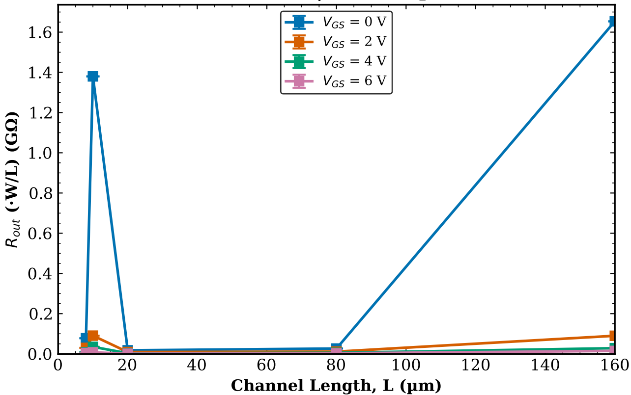
TFT3 Transistor 1 R_{out} vs L | W = 10\text{ }\mu\text{m}
